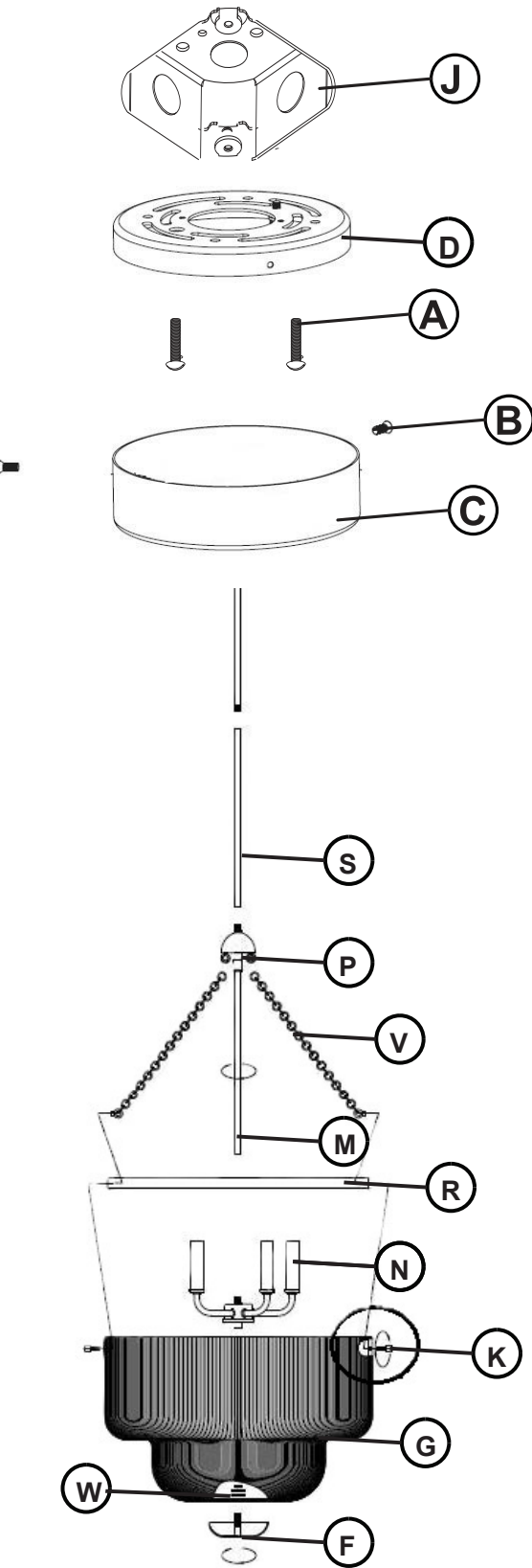
DRAWING 1 - MOUNTING
